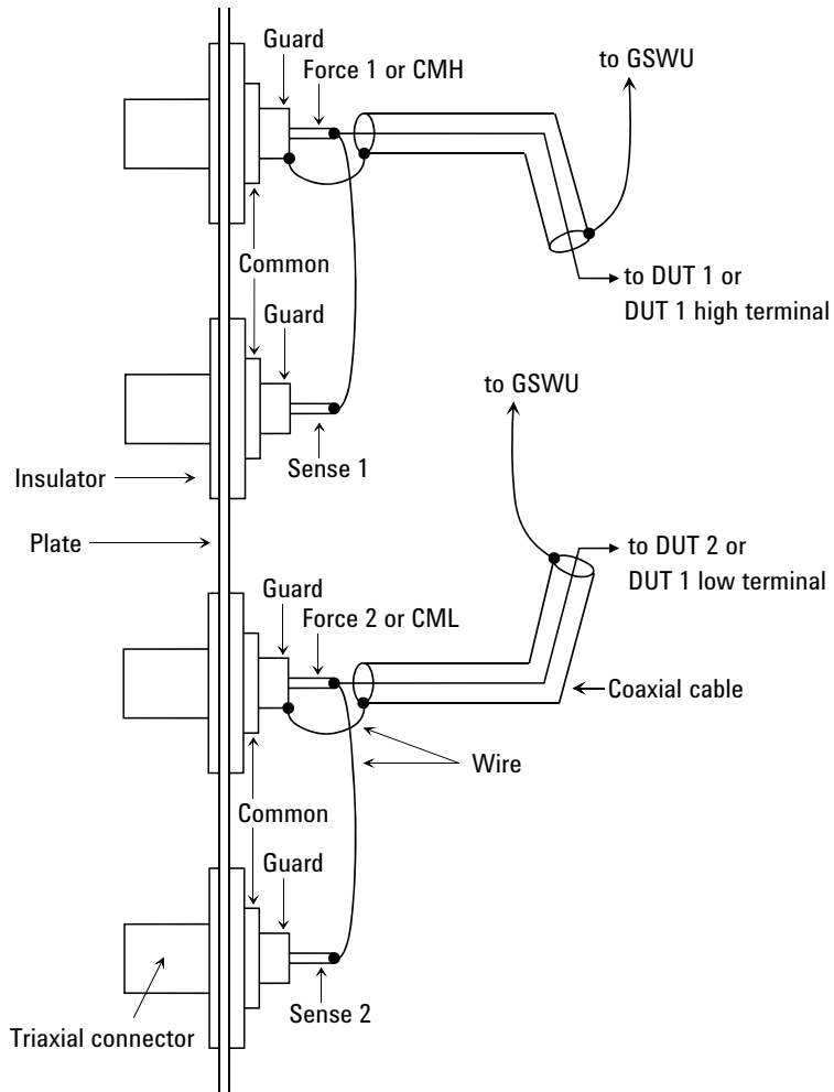
Figure 3-19 SCUU Output non-Kelvin Connection
