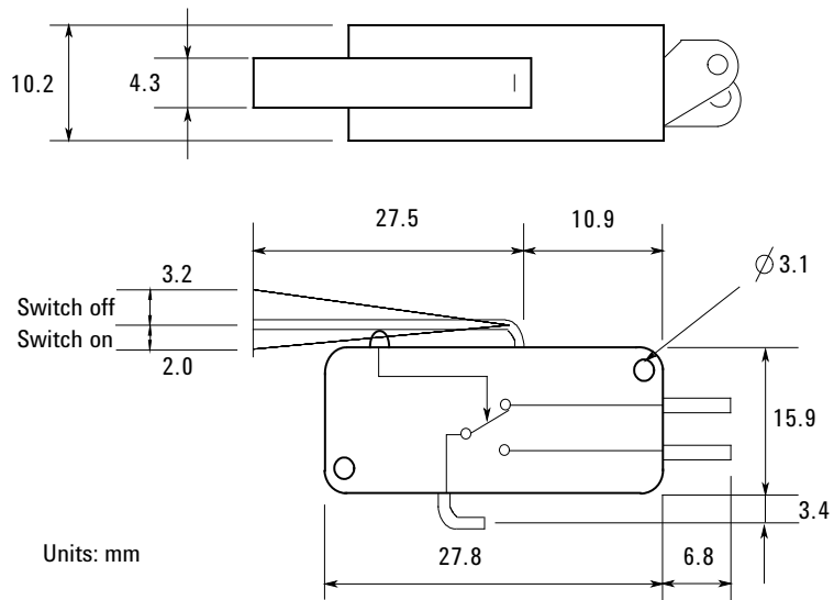
Dimensions of the Interlock Switch (3101-3241)
