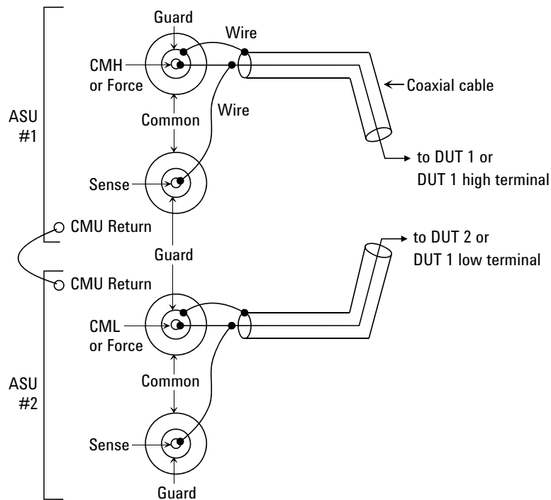
Figure 3-17 ASU Output non-Kelvin Connection
