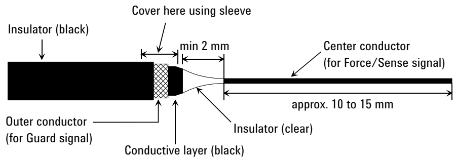
Figure 3-15 Coaxial Cable Cutting Example
