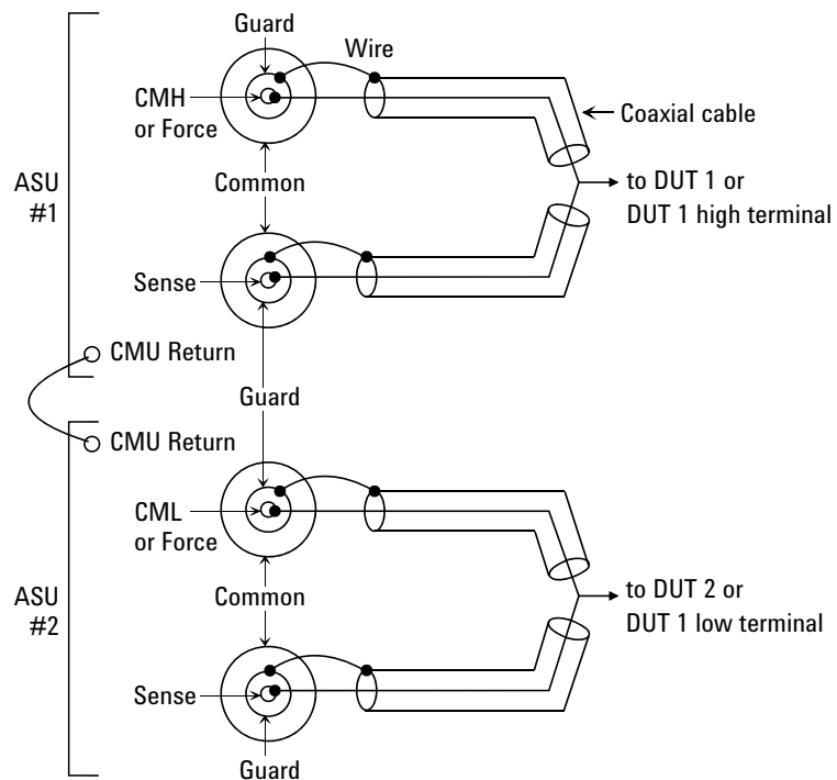
Figure 3-16 ASU Output Kelvin Connection (Remote Sensing)
